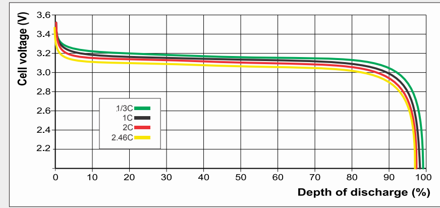
Discharging Curve
