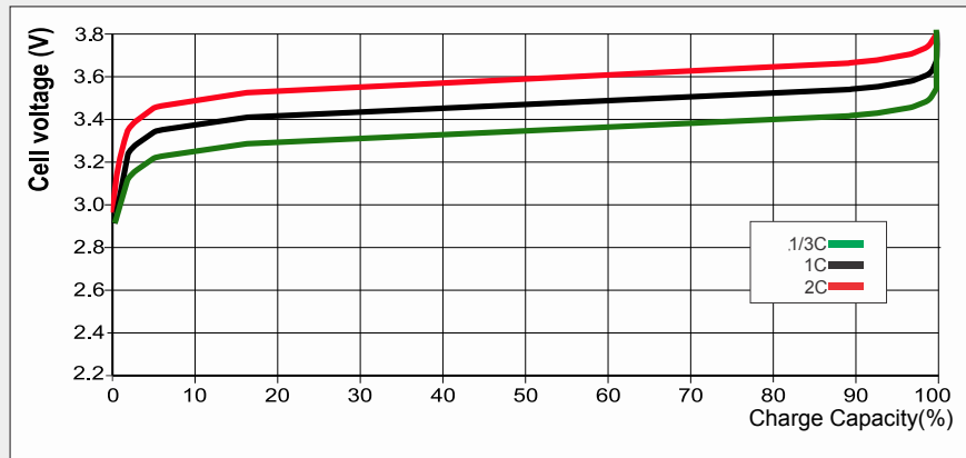
Charging Curve
